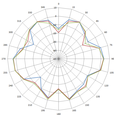
2.4GHz-E Plane
