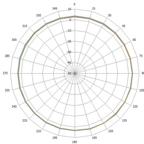
2.4GHz-H Plane
