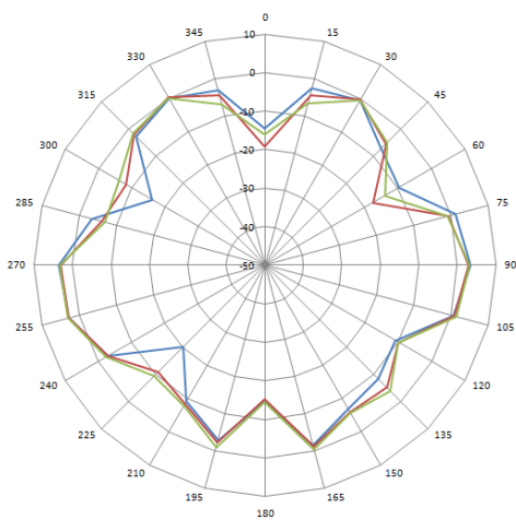
5GHz-E Plane
