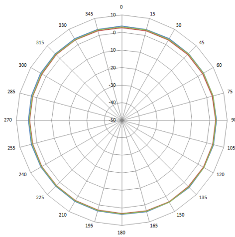
5GHz-H Plane
