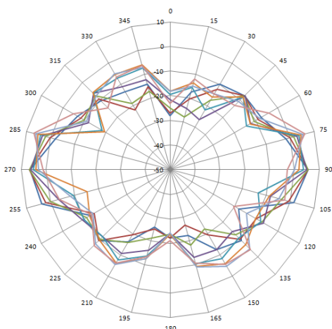
5GHz-E Plane
