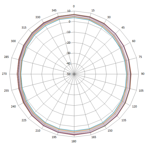
5GHz-H Plane
