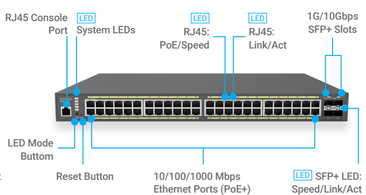
CloudSwitch L2Plus 48 PoE (ECS1552P)
